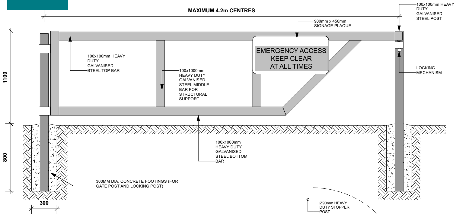
LOCKING MECHANISM
