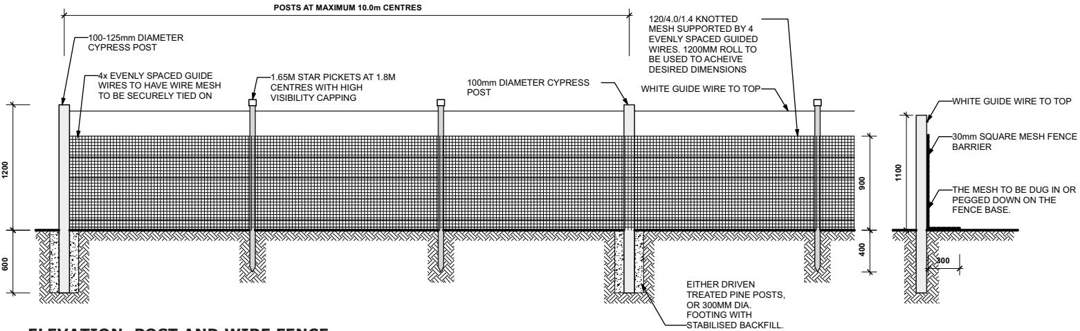
ELEVATION: POST AND WIRE FENCE
