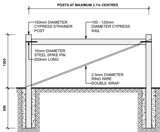
ELEVATION: STRAINER POST ASSEMBLY AND CORNER
