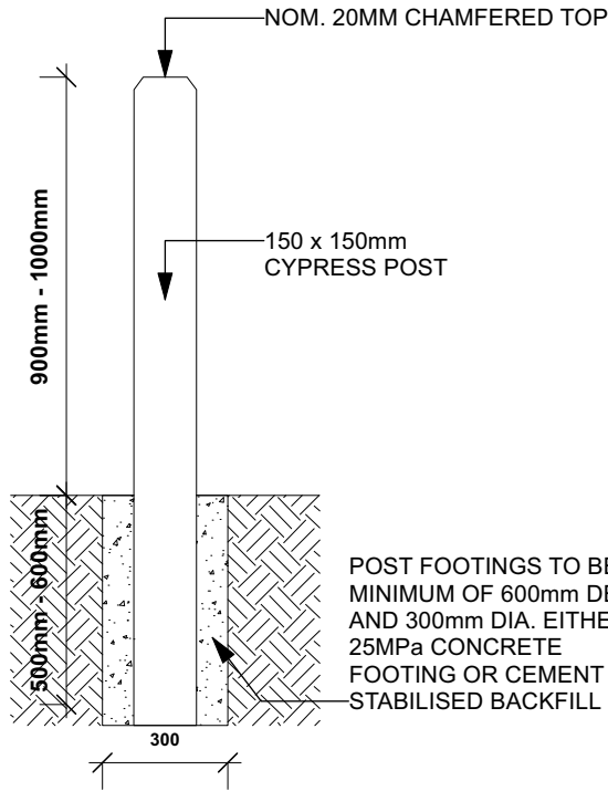
SECTION DETAIL
