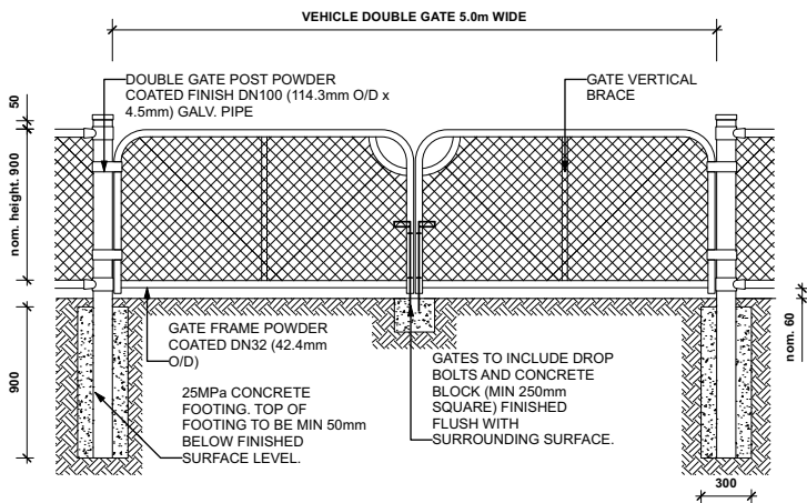
ELEVATION: SPORTSFIELD (CHAIN LINK MESH) DUAL ACCESS GATE
