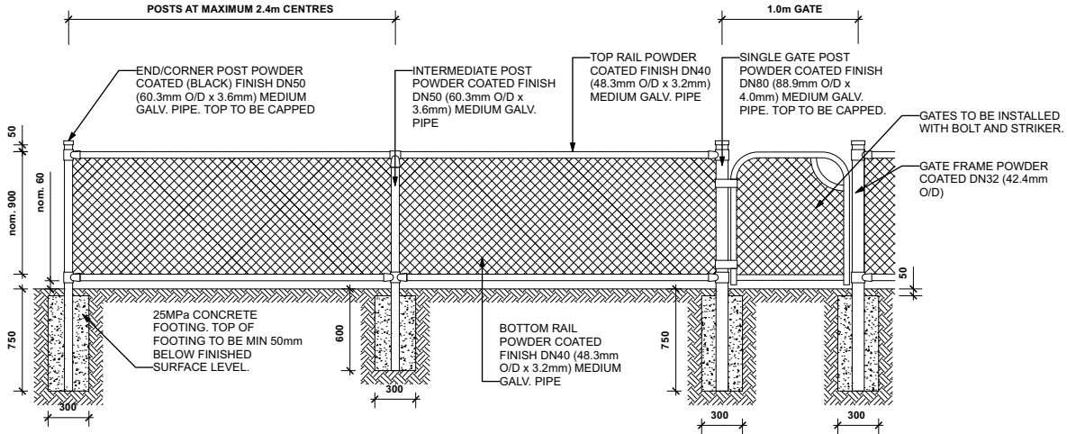
ELEVATION: SPORTSFIELD (CHAIN LINK MESH) FENCING WITH PEDESTRIAN GATE
